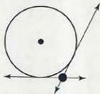
Two Tangents
