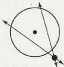
Two Secants
